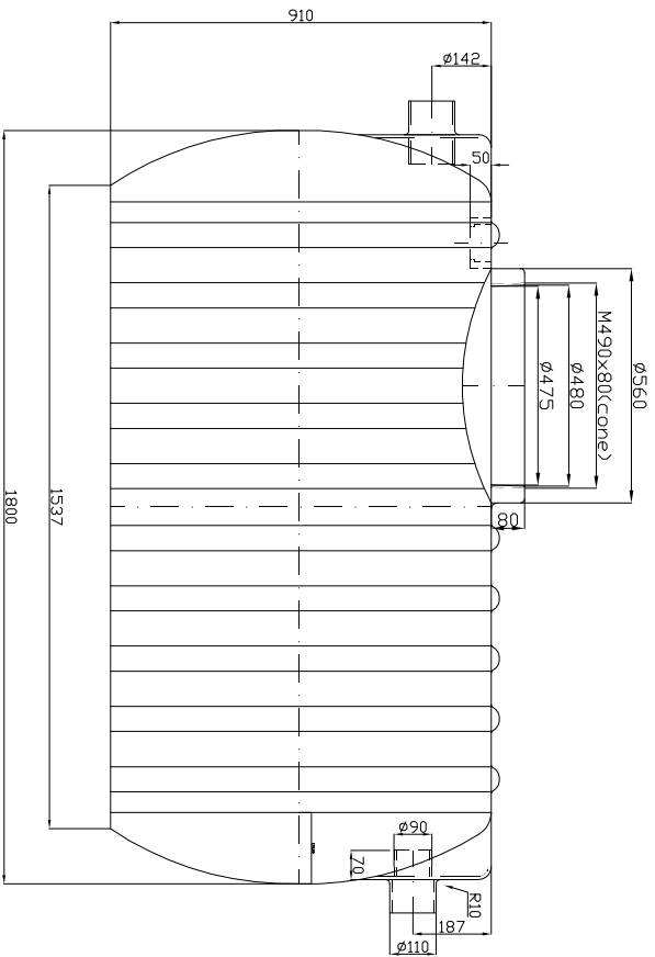
SEPTIC: FRONT VIEW
