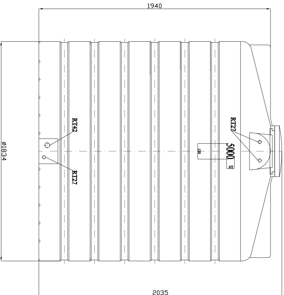
LEFT VIEW
