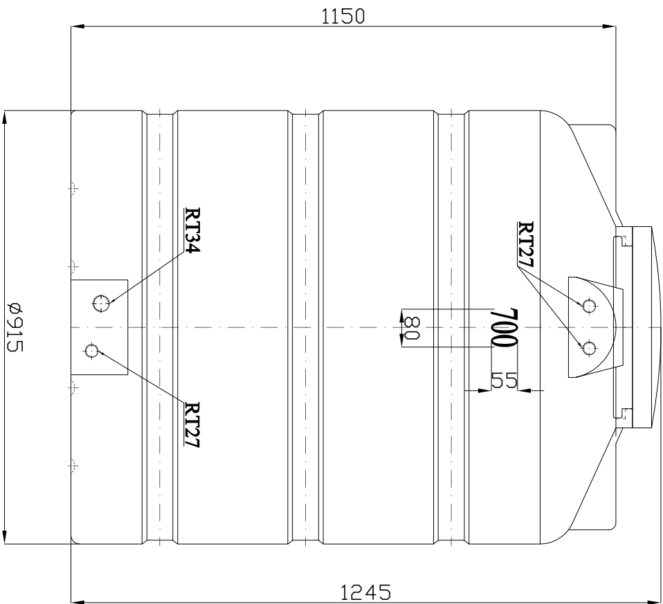
LEFT VIEW
