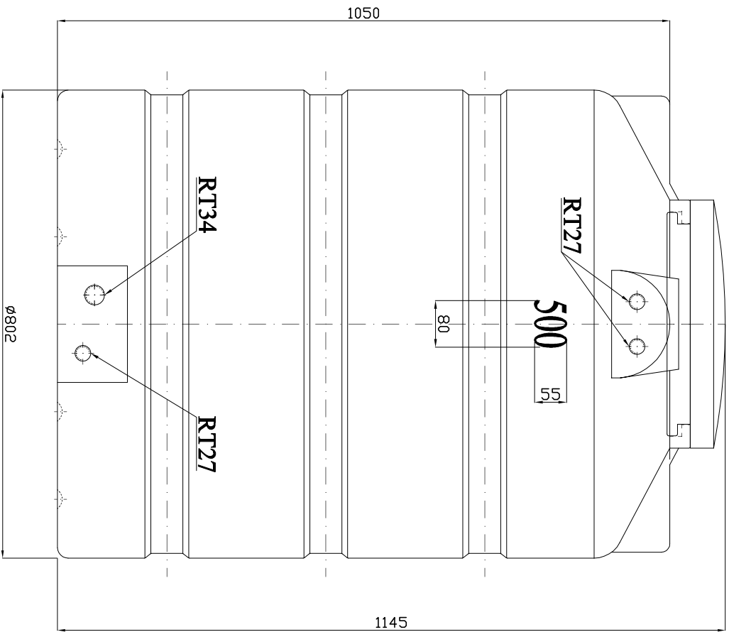
FRONT VIEW
