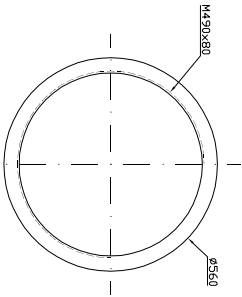
LID: BOTTOM VIEW
