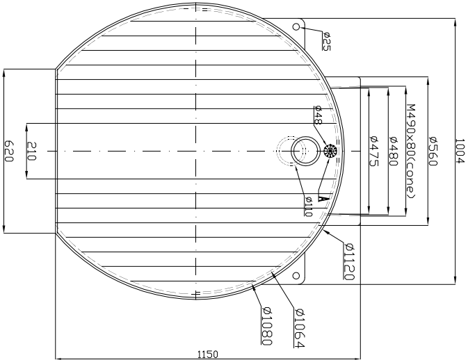
SEPTIC: LEFT VIEW
