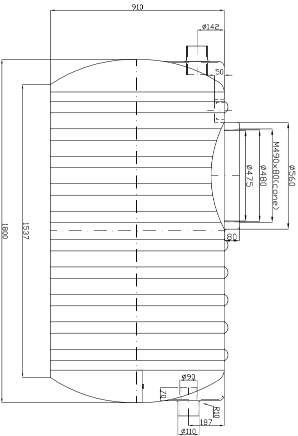
SEPTIC: FRONT VIEW
