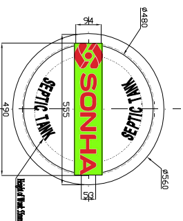
LID: TOP VIEW
