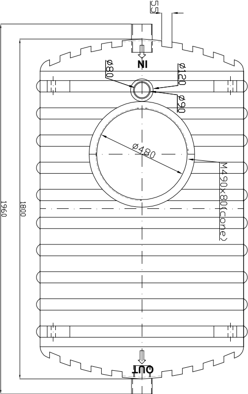
SEPTIC: TOP VIEW
