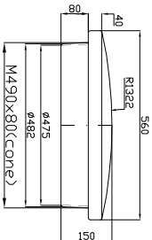
LID: FRONT VIEW
