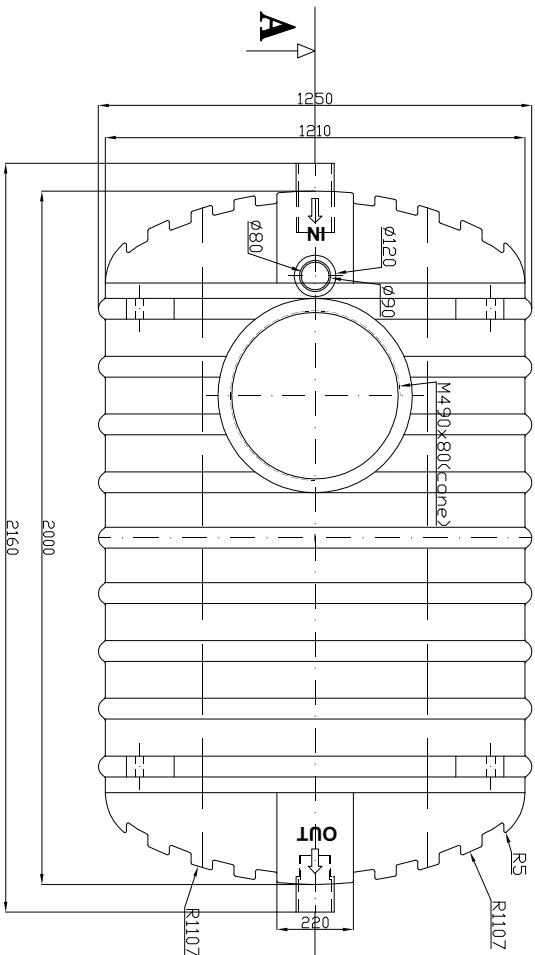
SEPTIC: TOP VIEW
