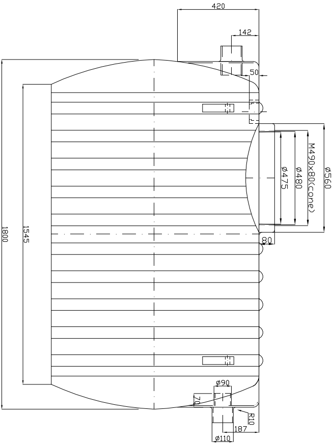
SEPTIC: FRONT VIEW
