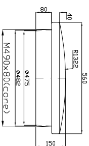
LID: FRONT VIEW
