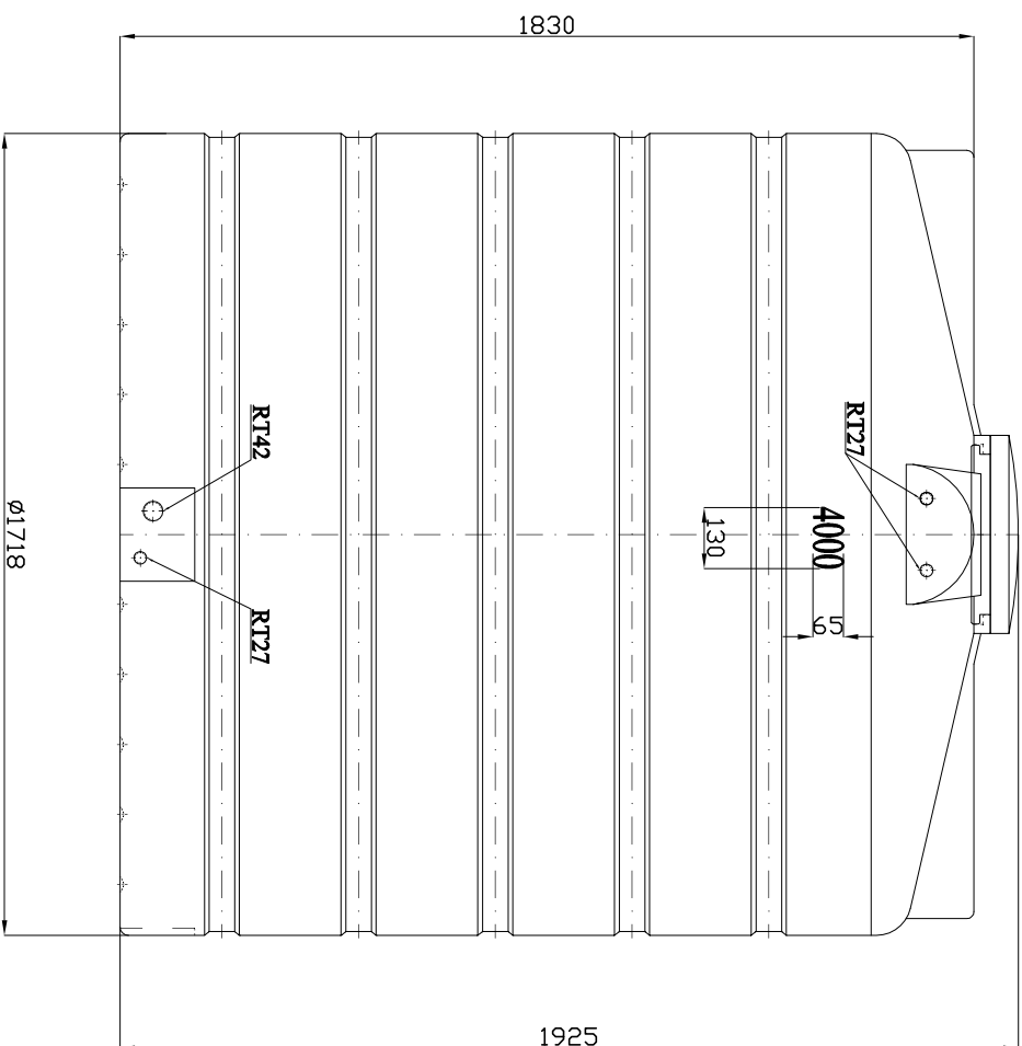
LEFT VIEW
